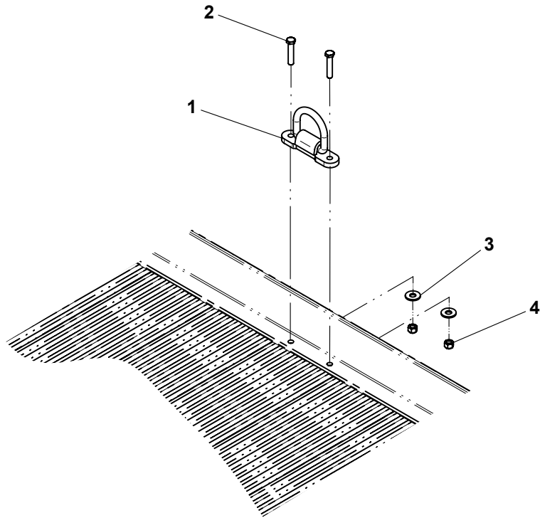
ALUMINUM DECK
