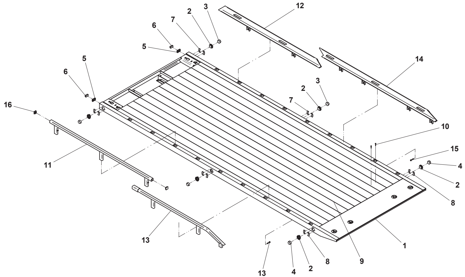
21' deck shown with optional removable steel rails on left side and optional aluminum removable rails on right side
