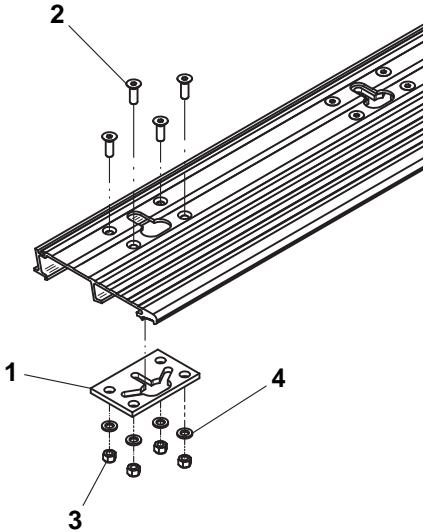
ALUMINUM DECKS
