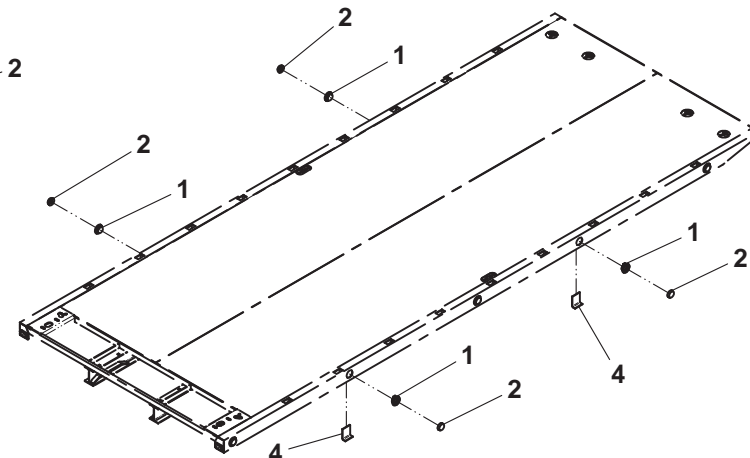
STEEL DECK
