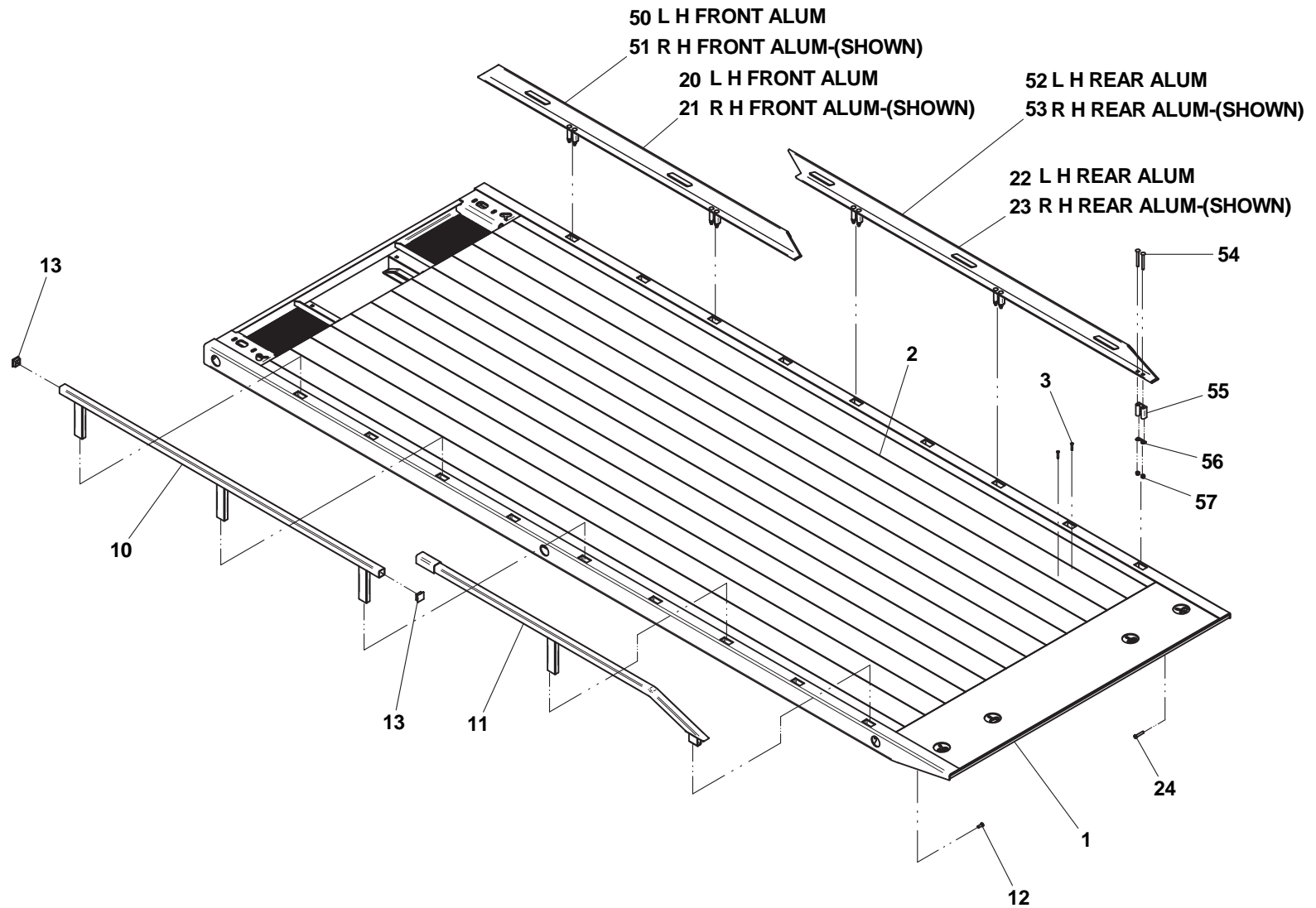
21' deck shown with optional removable steel rails on left side and optional aluminum removable rails on right side
