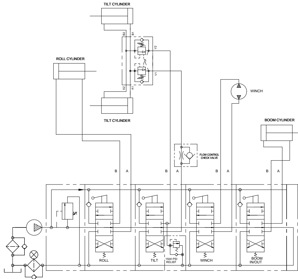
4 Bank Control Valve - Hydraulic Extended Boom Tow Options
