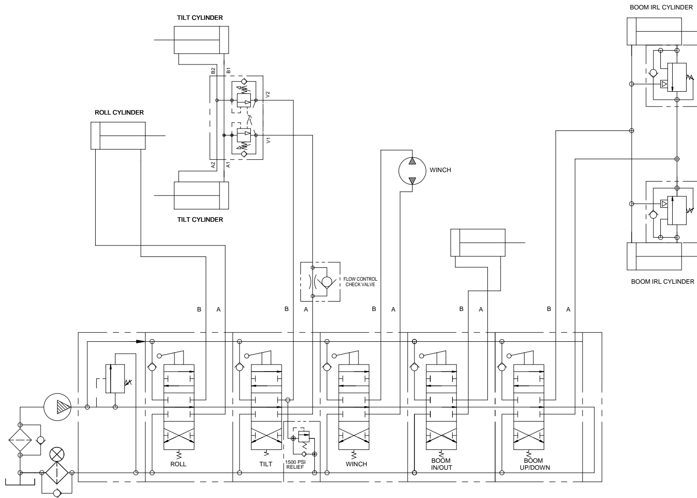
5 Bank Control Valve - IRL Tow Options
