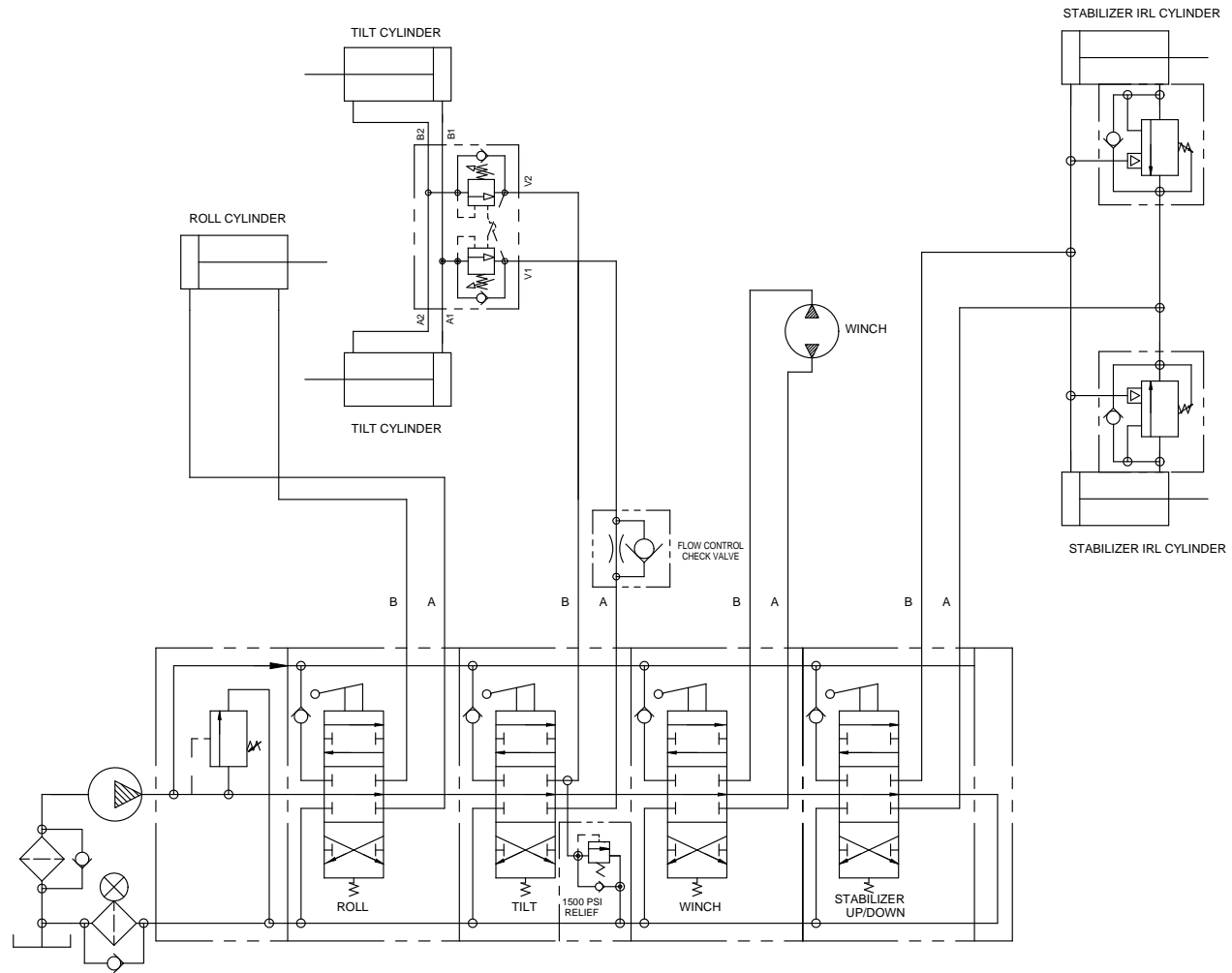
4 Bank Control Valve - Stabilizer with Tow Options
