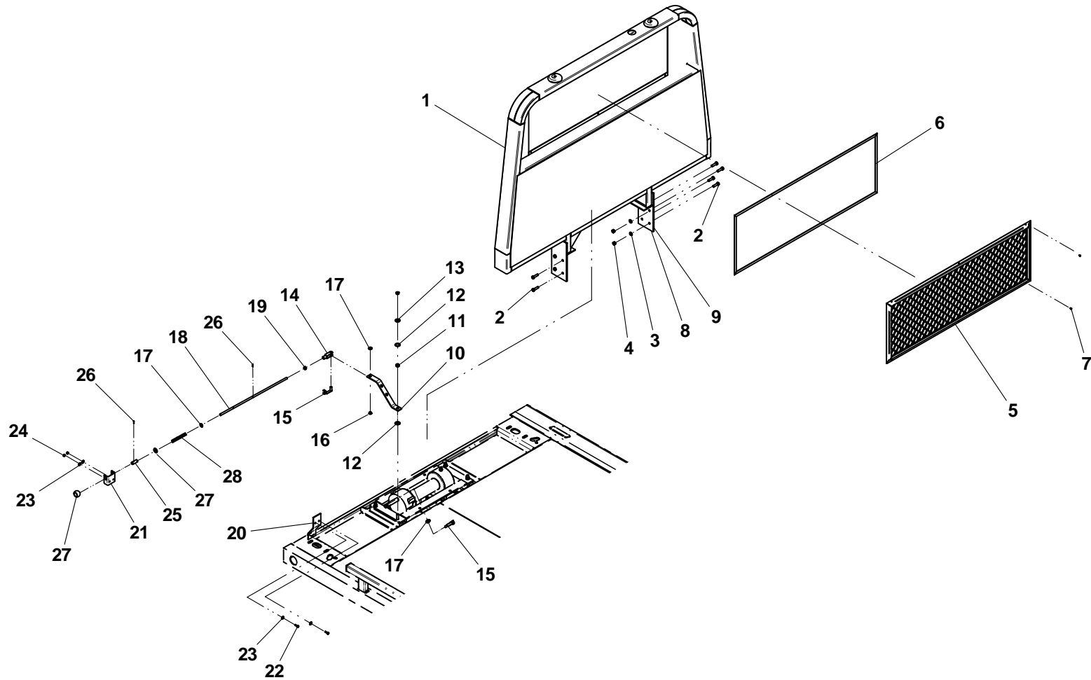
62.00" headboard shown with 10,000 lb worm gear winch
